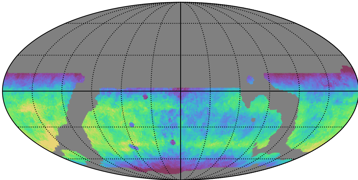
weather_cloudso20v3.4_10yrs WFD r band: Median fiveSigmaDepth
