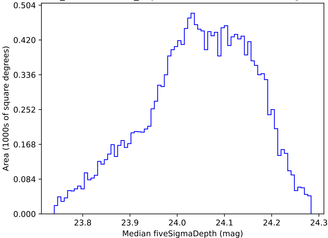
weather_cloudso20v3.4_10yrs WFD r band: Median fiveSigmaDepth
