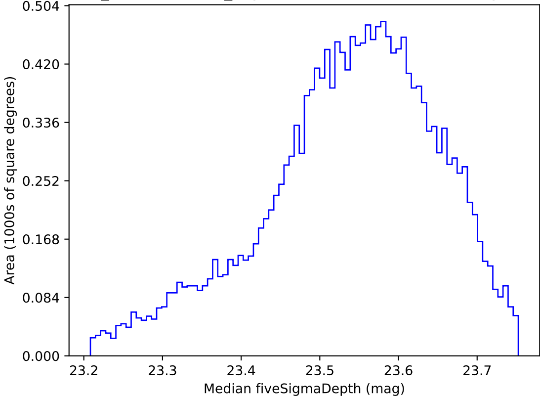
weather_cloudso20v3.4_10yrs WFD i band: Median fiveSigmaDepth
