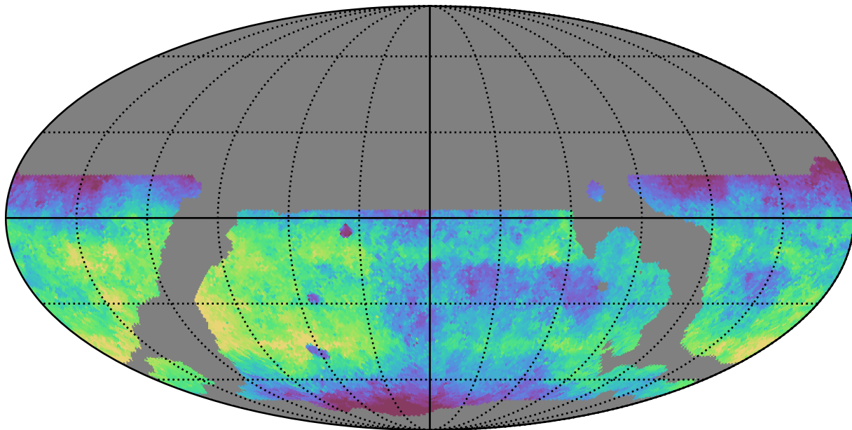
weather_cloudso20v3.4_10yrs WFD g band: Median fiveSigmaDepth
