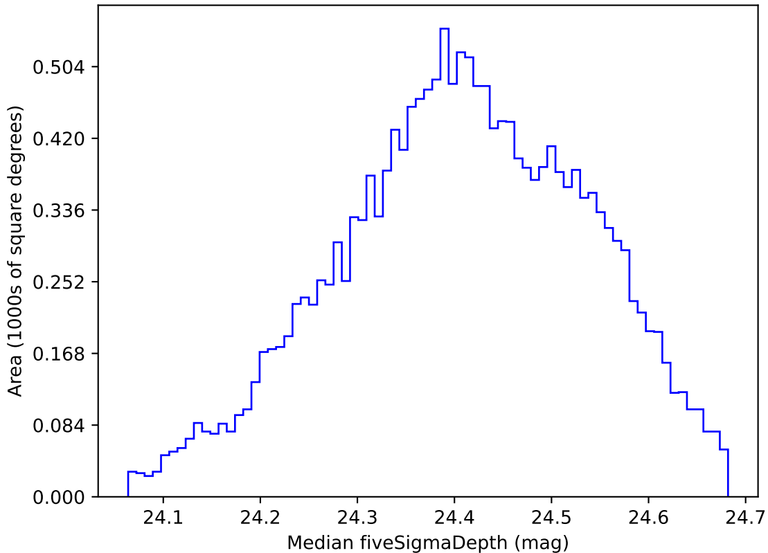
weather_cloudso20v3.4_10yrs WFD g band: Median fiveSigmaDepth
