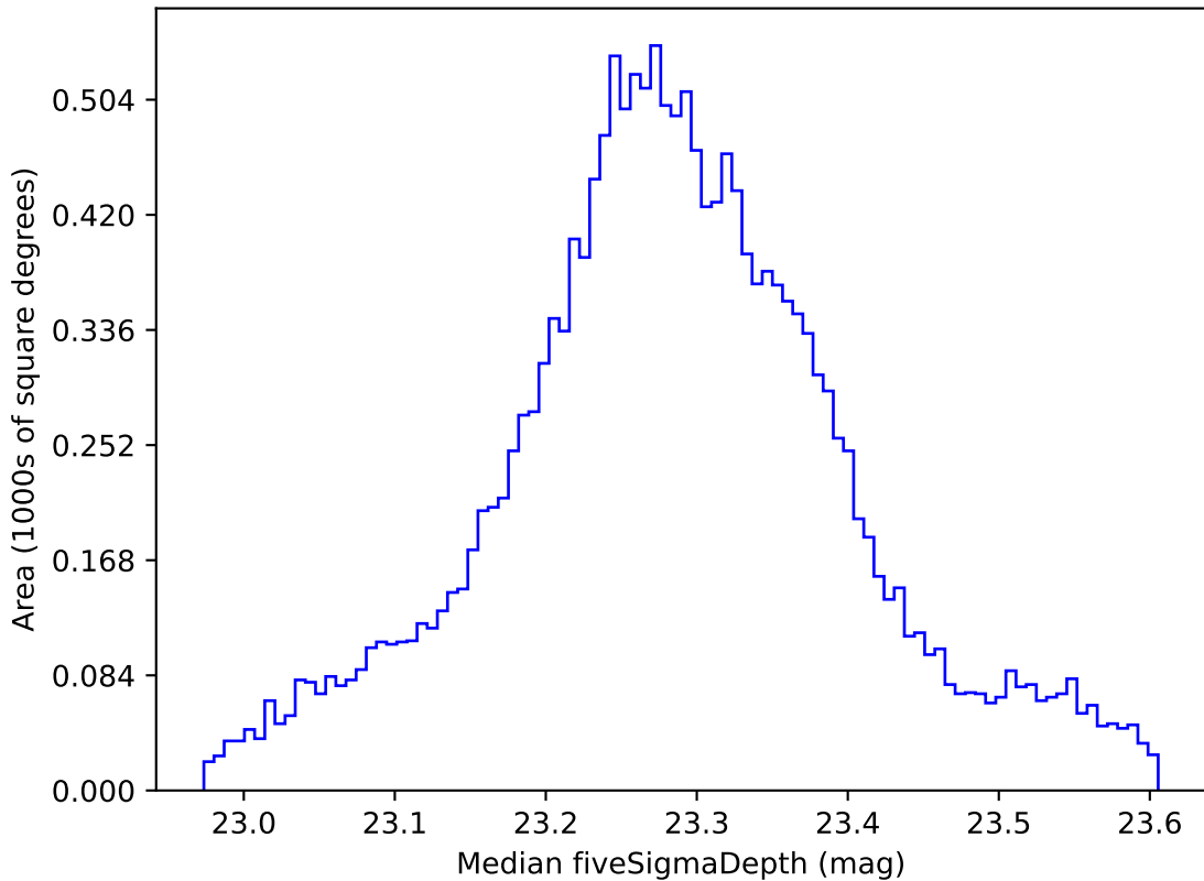
weather_cloudso20v3.4_10yrs WFD all bands: Median fiveSigmaDepth
