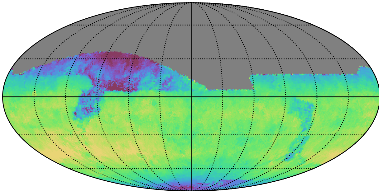
weather_cloudso20v3.4_10yrs All sky z band: Median fiveSigmaDepth
