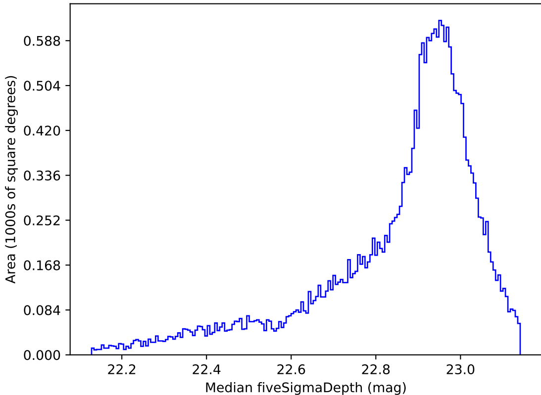
weather_cloudso20v3.4_10yrs All sky z band: Median fiveSigmaDepth
