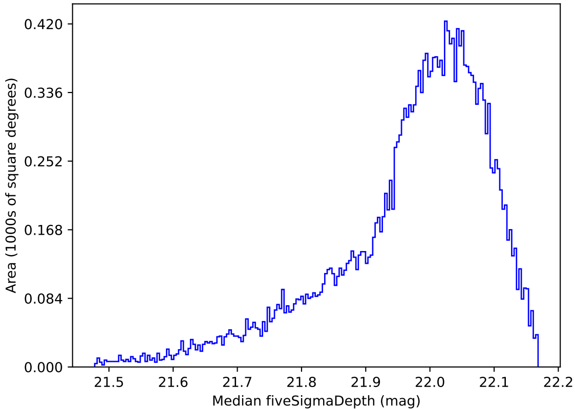
weather_cloudso20v3.4_10yrs All sky y band: Median fiveSigmaDepth
