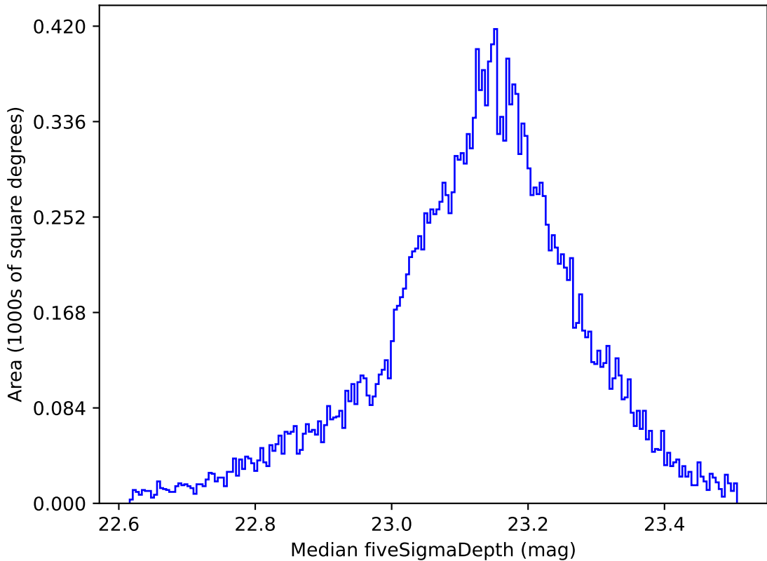
weather_cloudso20v3.4_10yrs All sky u band: Median fiveSigmaDepth
