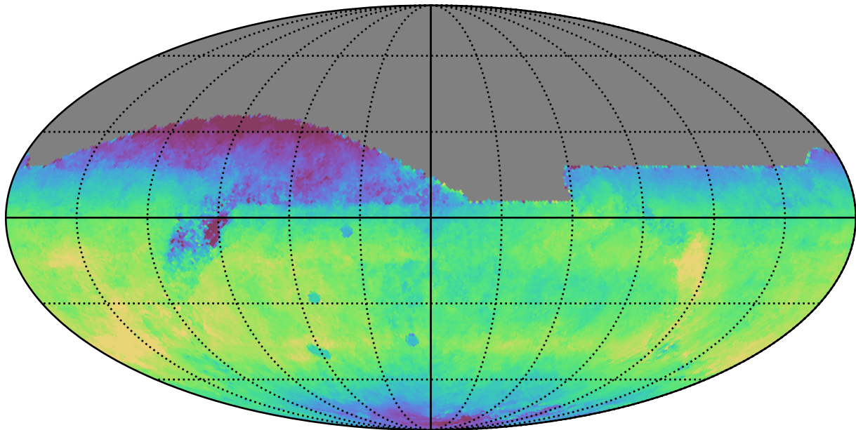
weather_cloudso20v3.4_10yrs All sky r band: Median fiveSigmaDepth
