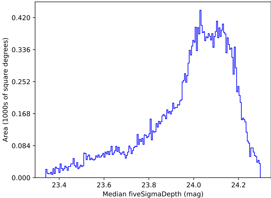
weather_cloudso20v3.4_10yrs All sky r band: Median fiveSigmaDepth
