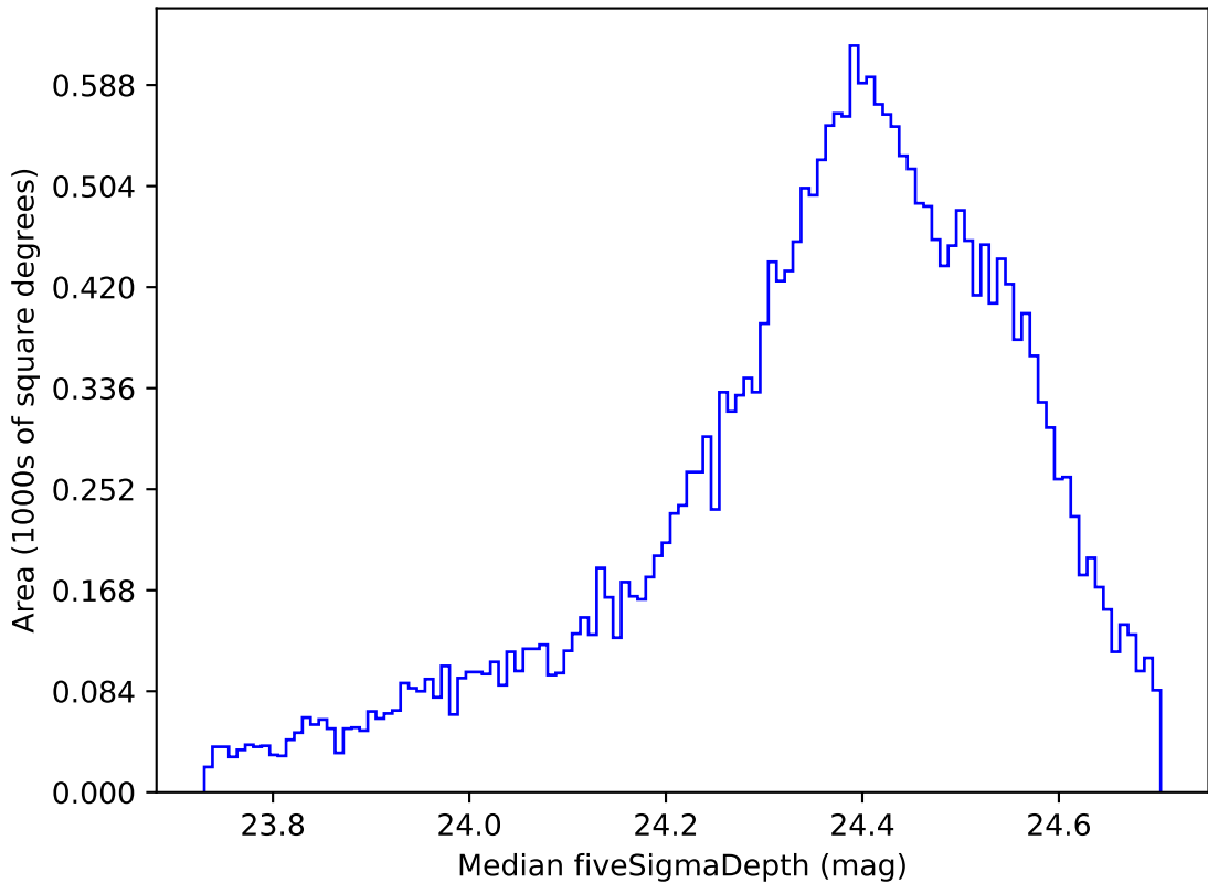
weather_cloudso20v3.4_10yrs All sky g band: Median fiveSigmaDepth
