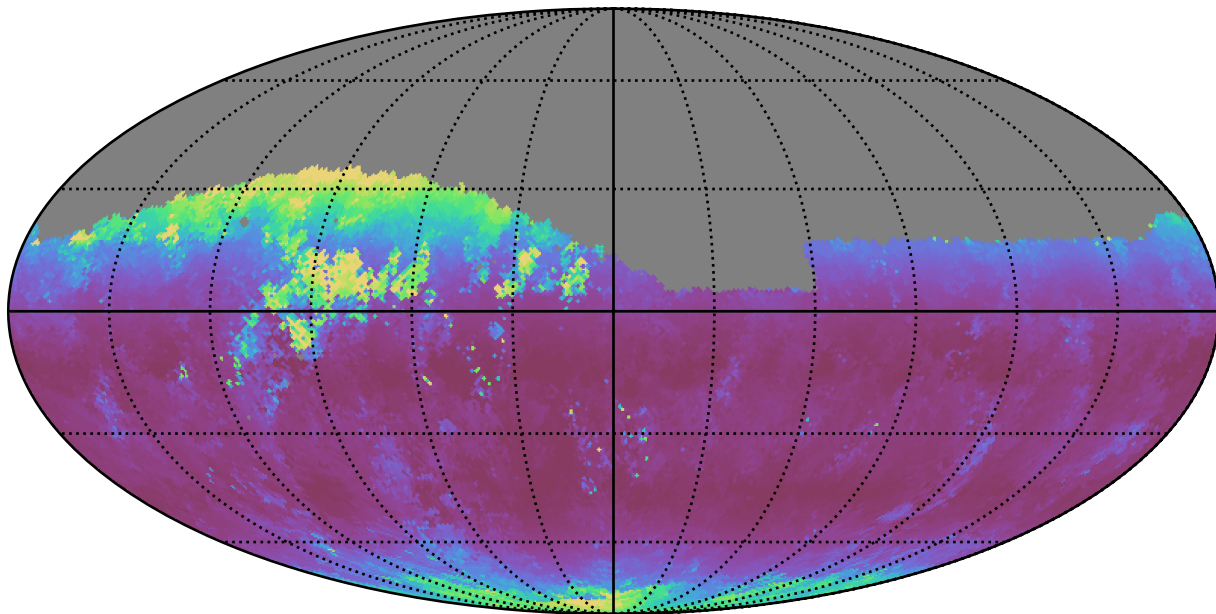
weather_cloudso20v3.4_10yrs Yr 1 z band: Median airmass
