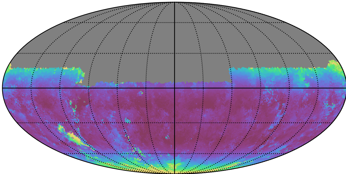
weather_cloudso20v3.4_10yrs Yr 1 y band: Median airmass
