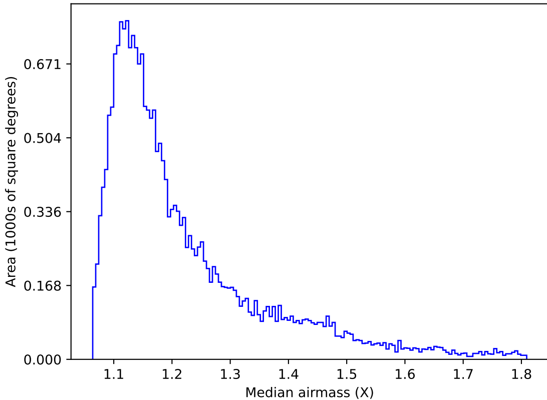
weather_cloudso20v3.4_10yrs Yr 1 y band: Median airmass
