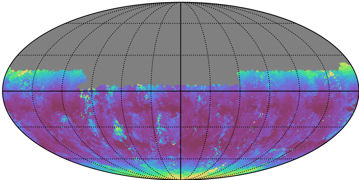
weather_cloudso20v3.4_10yrs Yr 1 u band: Median airmass
