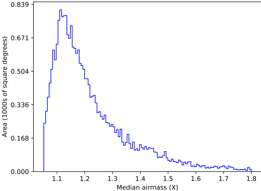
weather_cloudso20v3.4_10yrs Yr 1 u band: Median airmass
