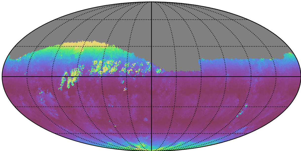
weather_cloudso20v3.4_10yrs Yr 1 r band: Median airmass
