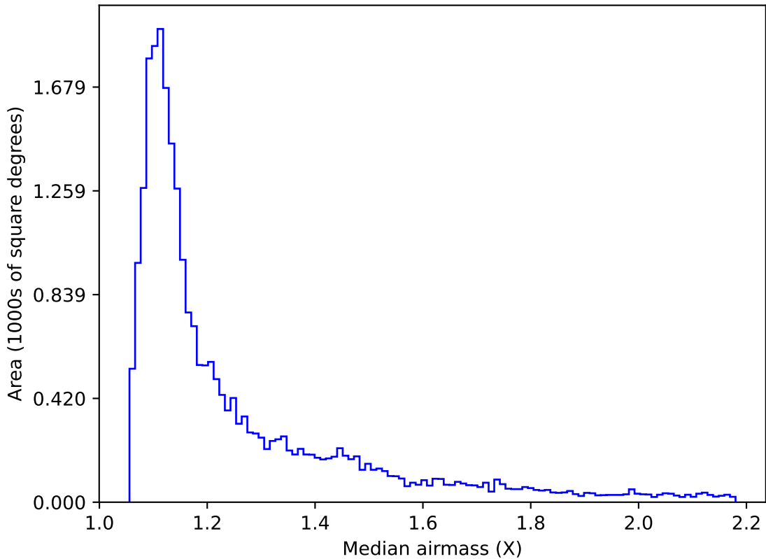
weather_cloudso20v3.4_10yrs Yr 1 r band: Median airmass
