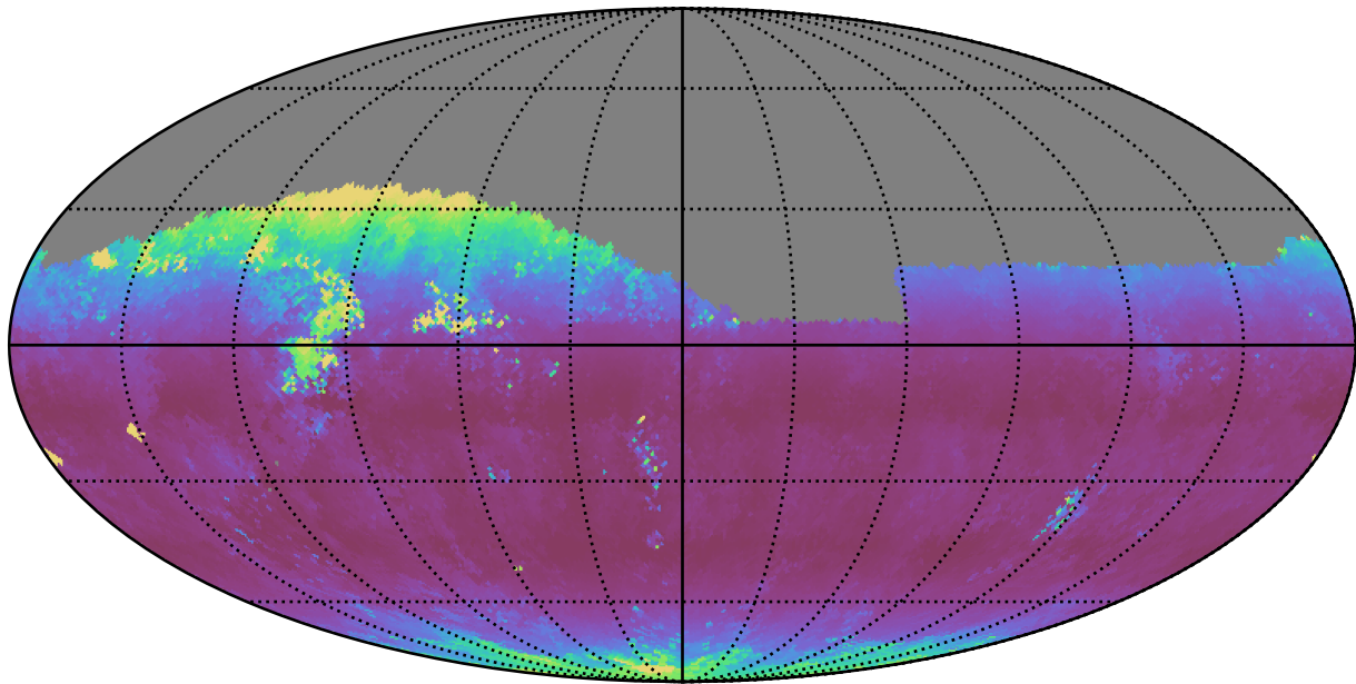
weather_cloudso20v3.4_10yrs Yr 1 i band: Median airmass
