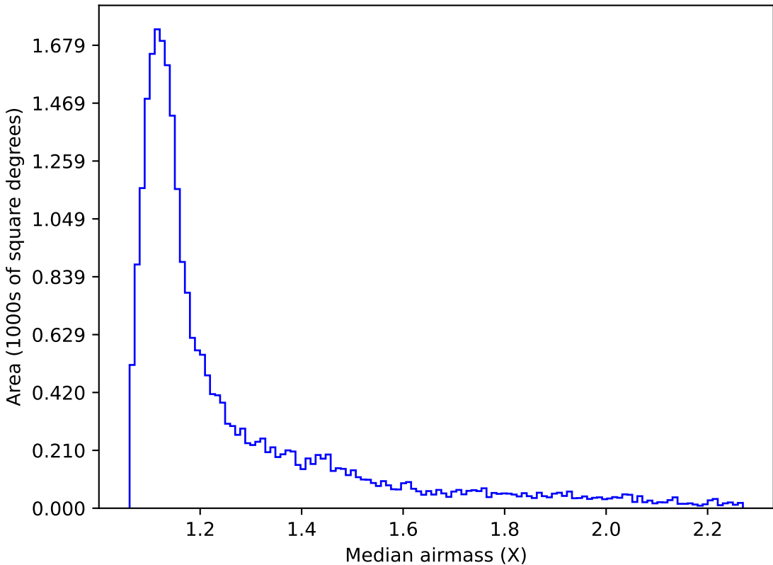
weather_cloudso20v3.4_10yrs Yr 1 i band: Median airmass
