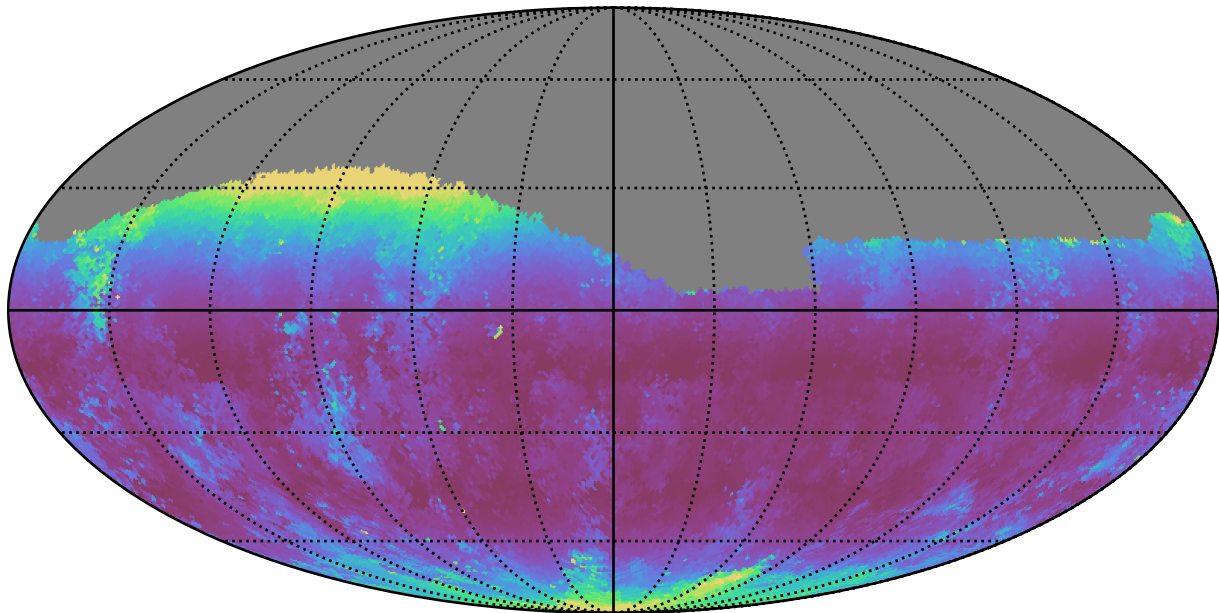
weather_cloudso20v3.4_10yrs Yr 1 g band: Median airmass
