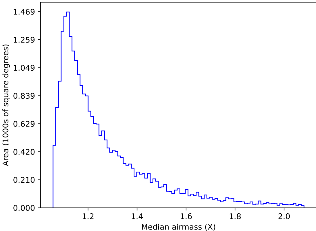
weather_cloudso20v3.4_10yrs Yr 1 g band: Median airmass
