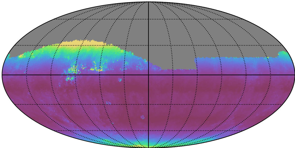
weather_cloudso20v3.4_10yrs Yr 1 all bands: Median airmass
