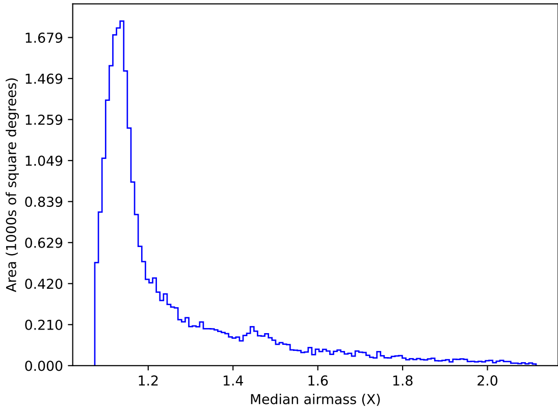
weather_cloudso20v3.4_10yrs Yr 1 all bands: Median airmass
