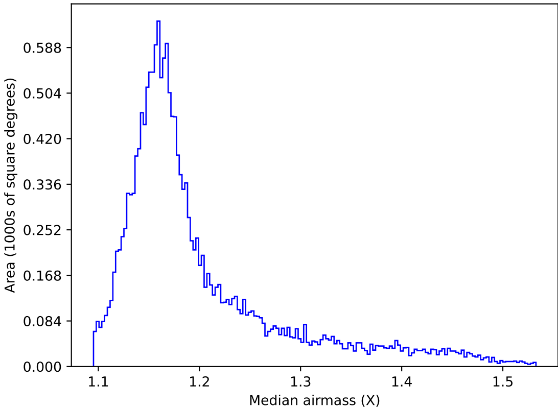
weather_cloudso20v3.4_10yrs WFD z band: Median airmass
