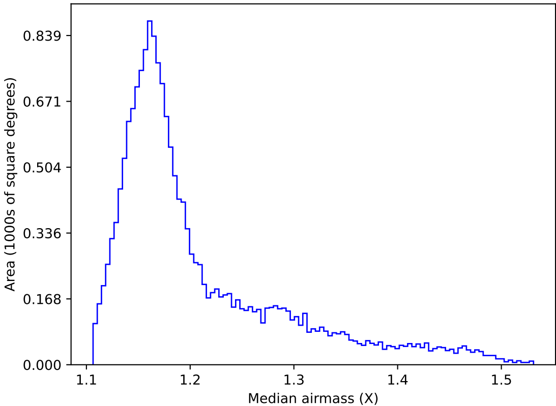
weather_cloudso20v3.4_10yrs WFD y band: Median airmass
