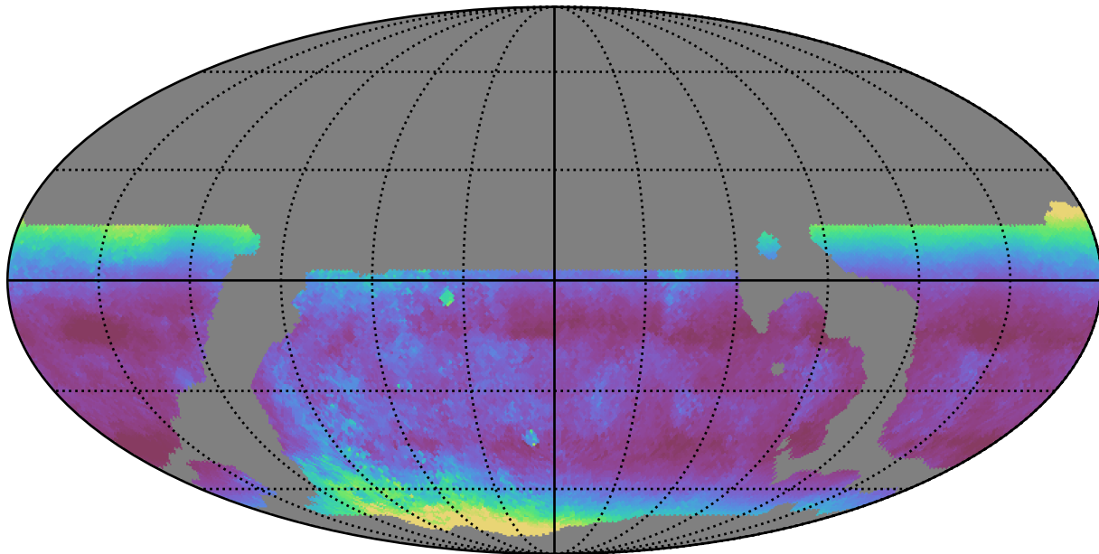
weather_cloudso20v3.4_10yrs WFD u band: Median airmass
