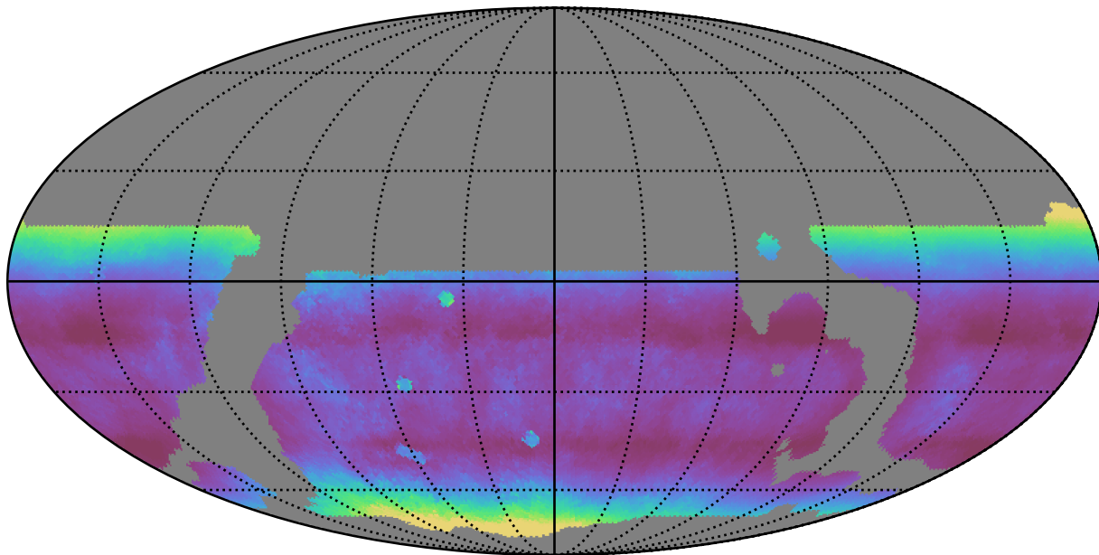
weather_cloudso20v3.4_10yrs WFD r band: Median airmass
