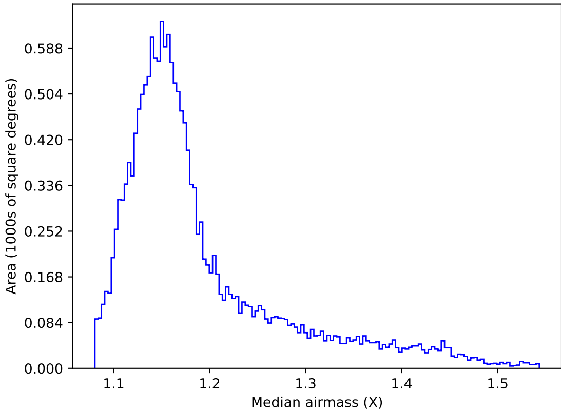
weather_cloudso20v3.4_10yrs WFD r band: Median airmass
