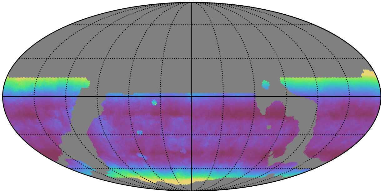
weather_cloudso20v3.4_10yrs WFD i band: Median airmass
