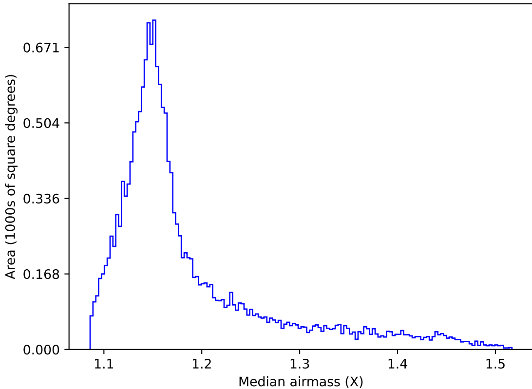
weather_cloudso20v3.4_10yrs WFD i band: Median airmass
