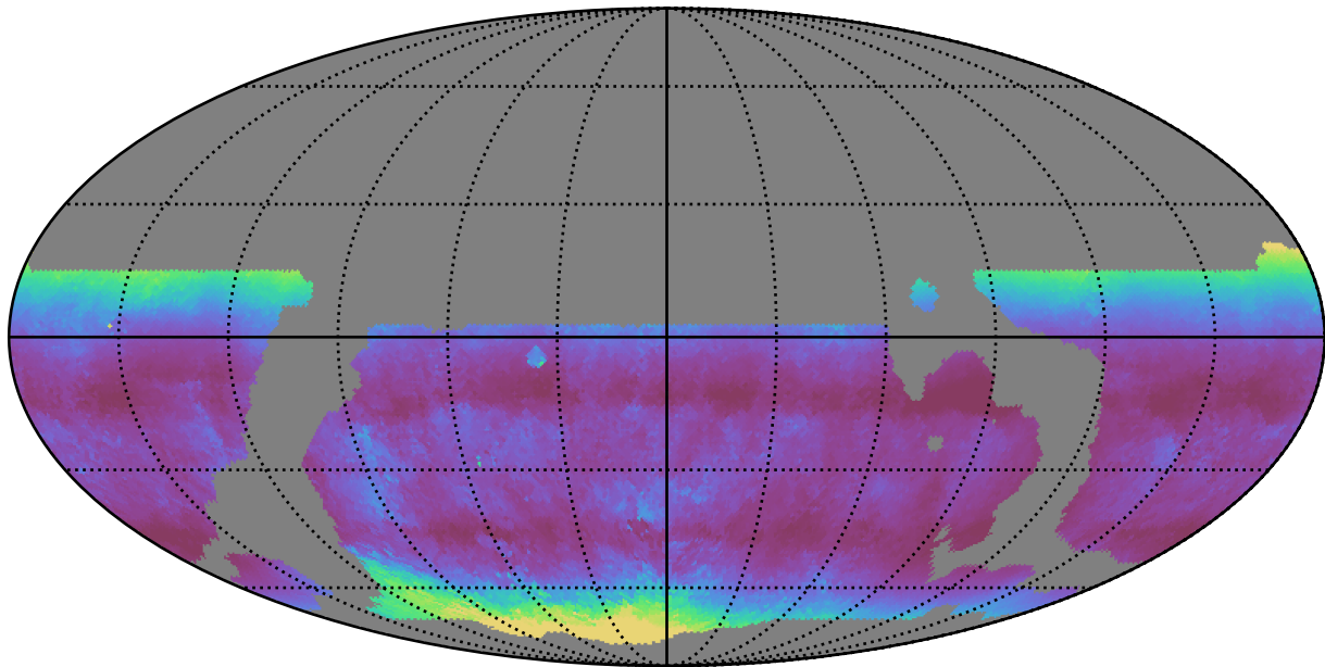
weather_cloudso20v3.4_10yrs WFD g band: Median airmass
