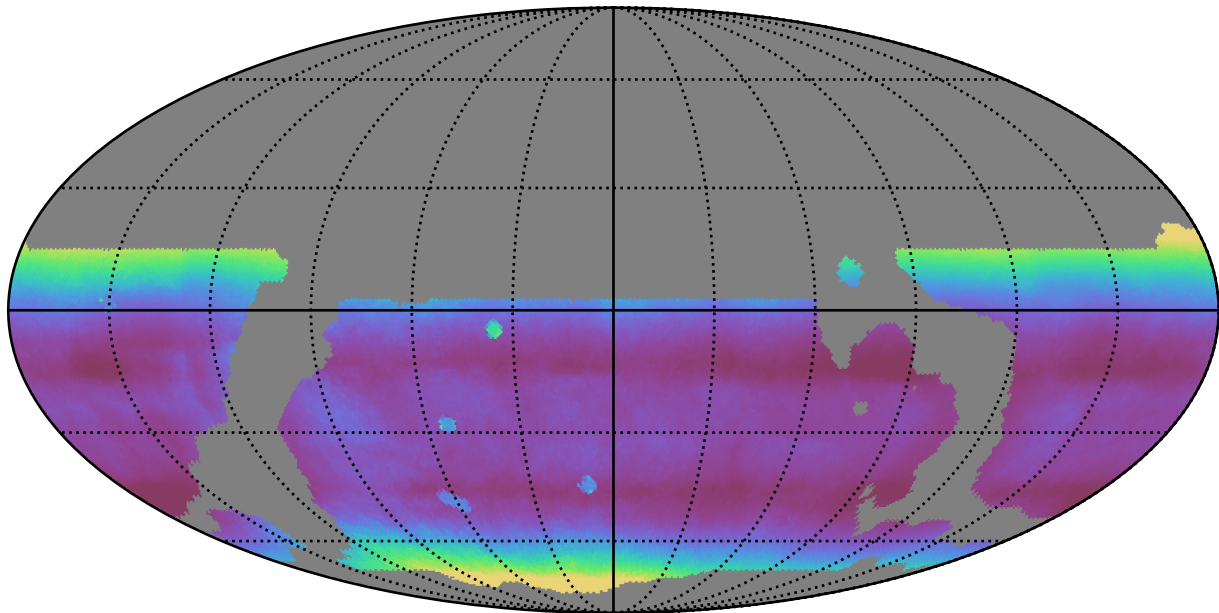
weather_cloudso20v3.4_10yrs WFD all bands: Median airmass
