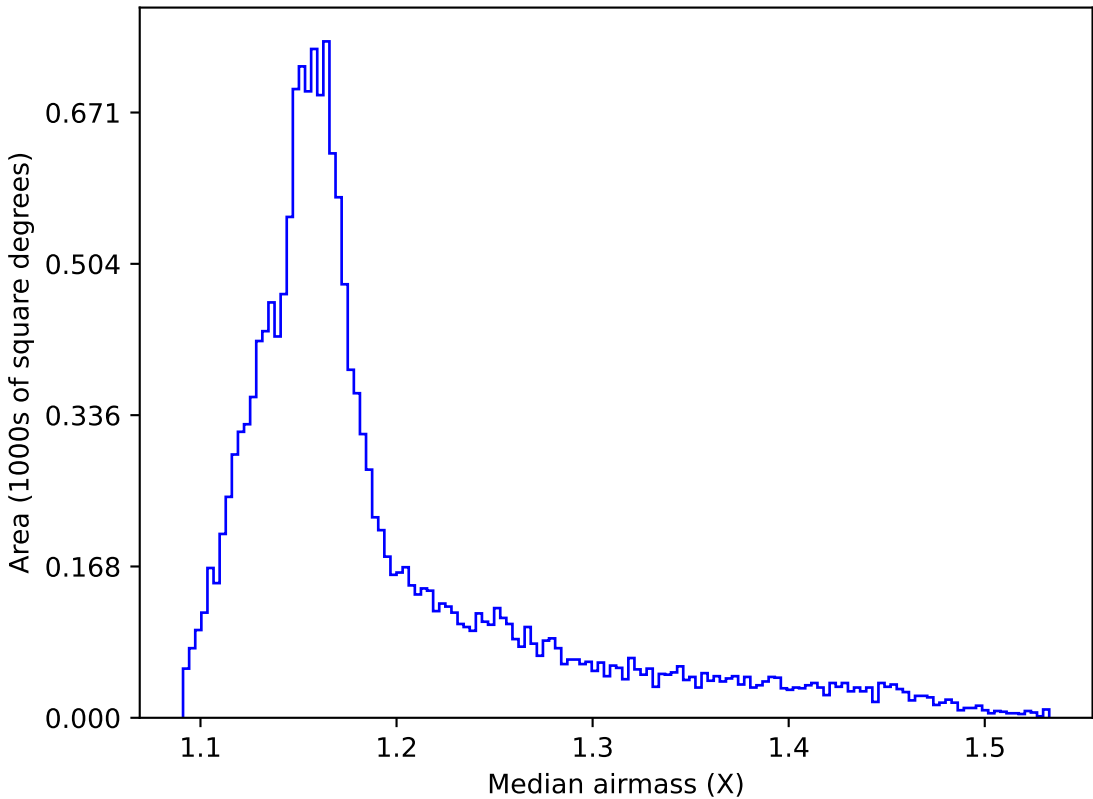
weather_cloudso20v3.4_10yrs WFD all bands: Median airmass
