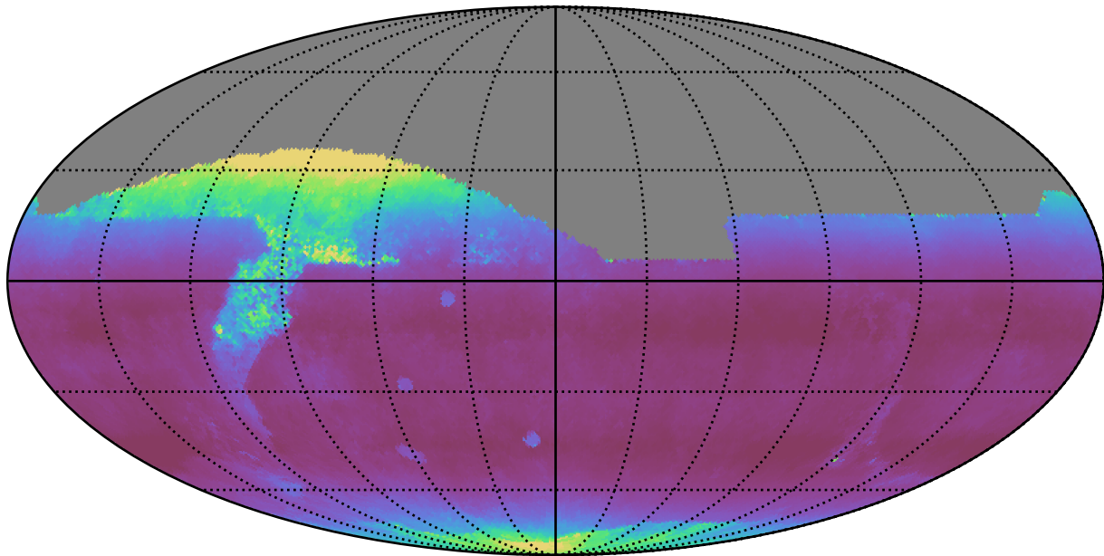
weather_cloudso20v3.4_10yrs All sky z band: Median airmass
