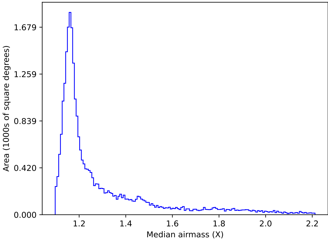
weather_cloudso20v3.4_10yrs All sky z band: Median airmass
