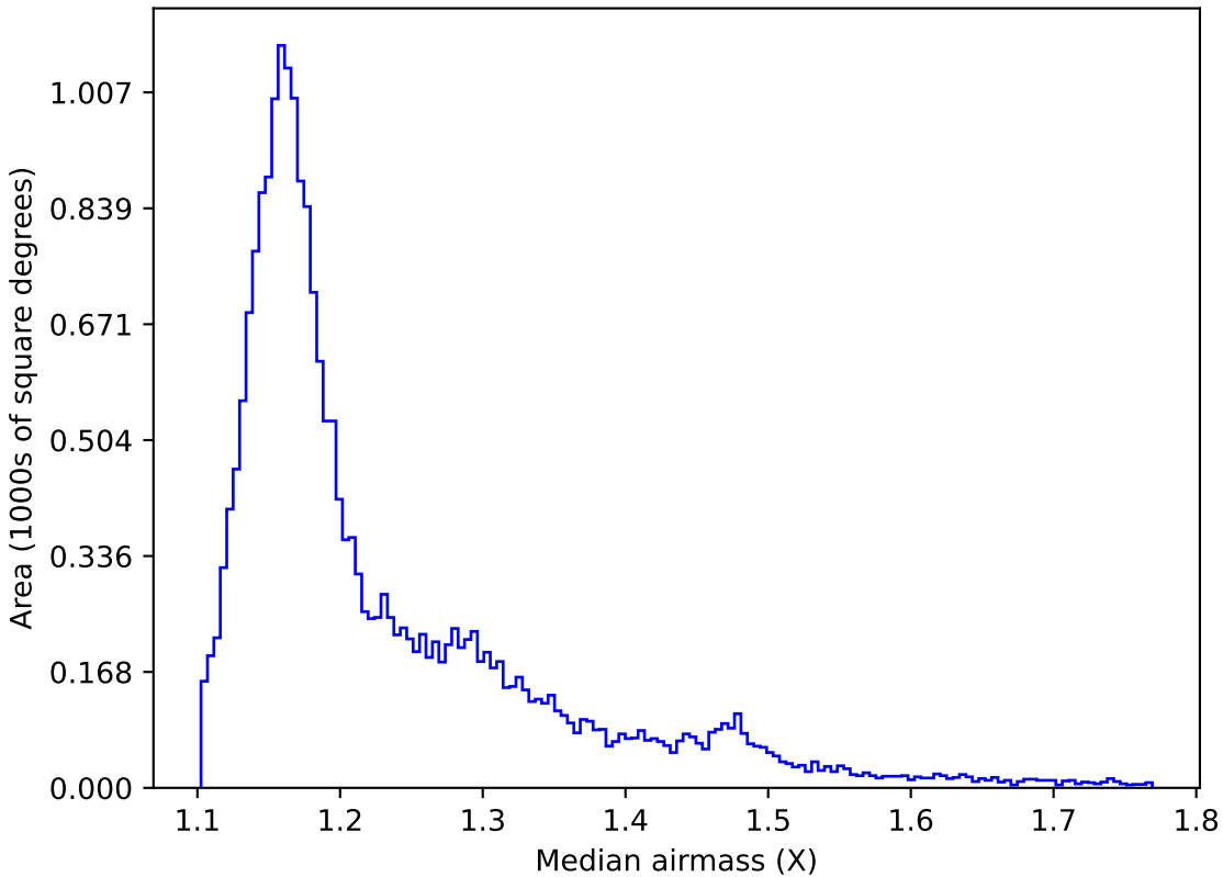
weather_cloudso20v3.4_10yrs All sky y band: Median airmass
