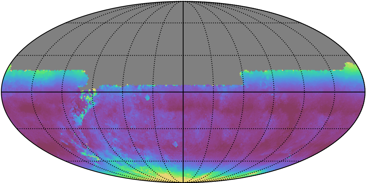
weather_cloudso20v3.4_10yrs All sky u band: Median airmass
