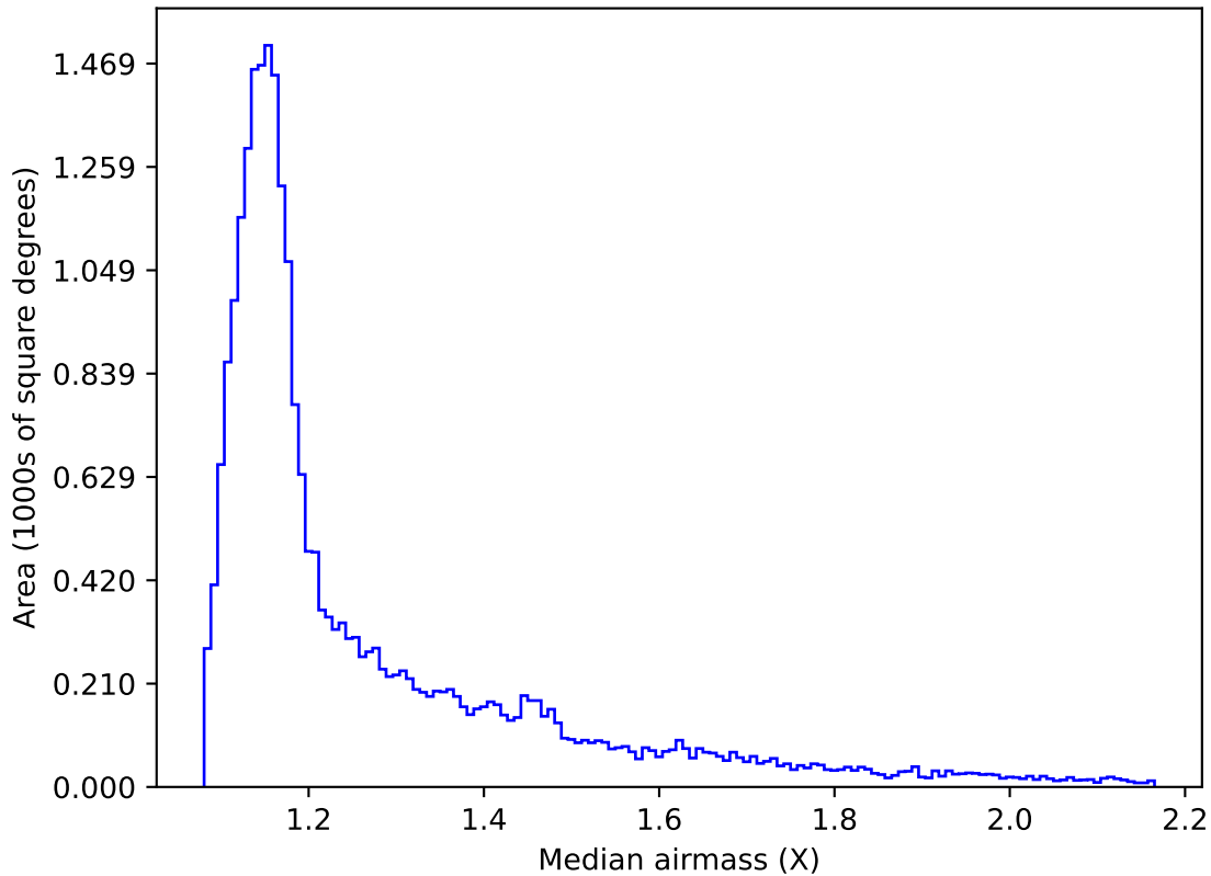
weather_cloudso20v3.4_10yrs All sky r band: Median airmass
