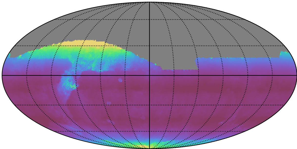
weather_cloudso20v3.4_10yrs All sky i band: Median airmass
