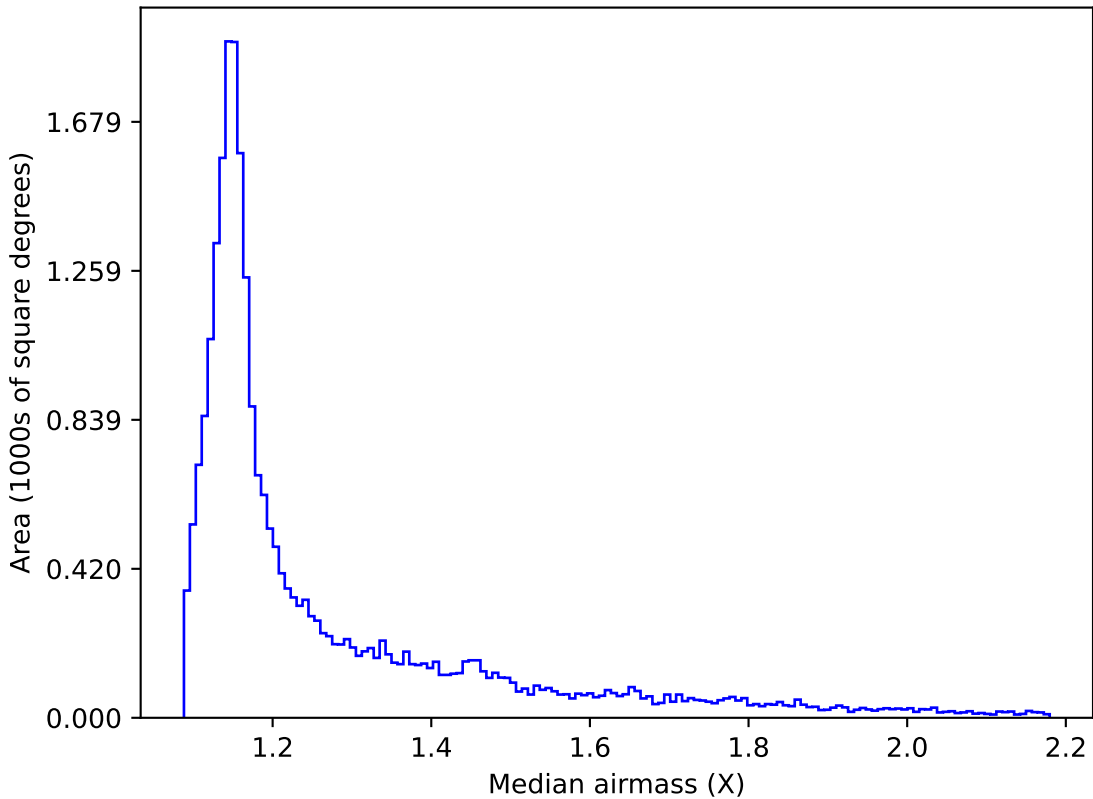
weather_cloudso20v3.4_10yrs All sky i band: Median airmass
