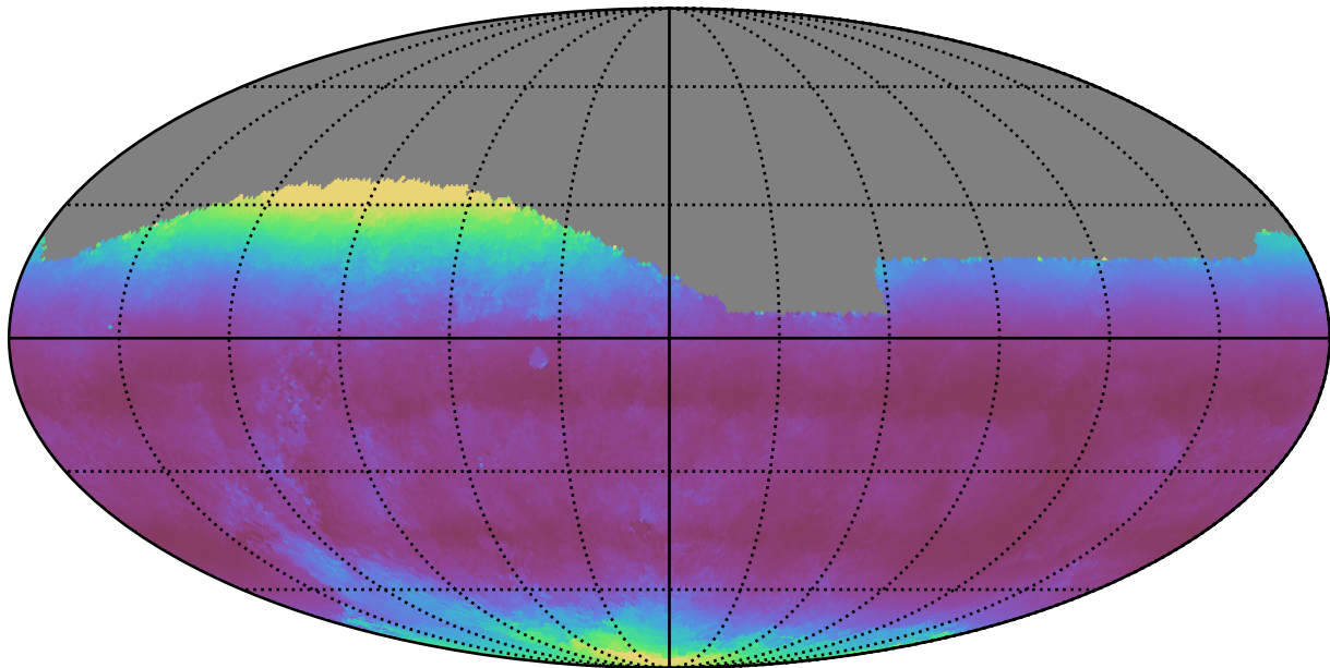
weather_cloudso20v3.4_10yrs All sky g band: Median airmass
