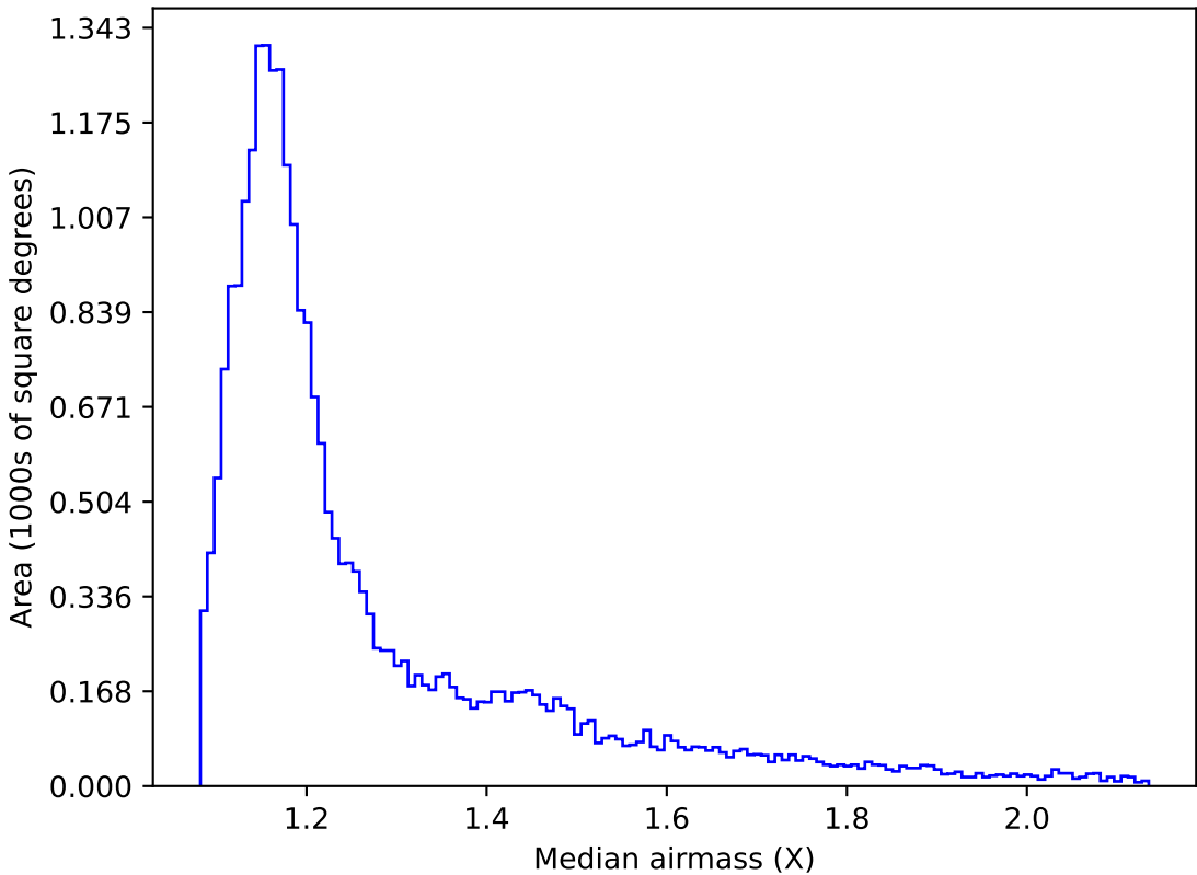
weather_cloudso20v3.4_10yrs All sky g band: Median airmass
