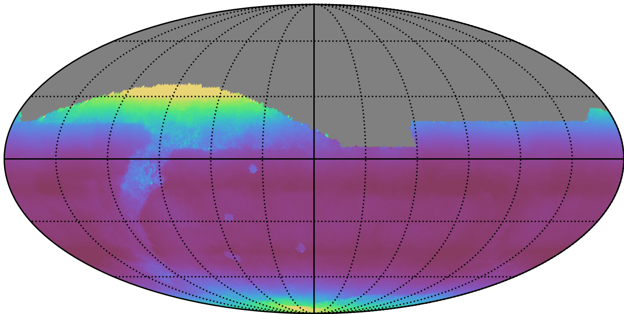
weather_cloudso20v3.4_10yrs All sky all bands: Median airmass
