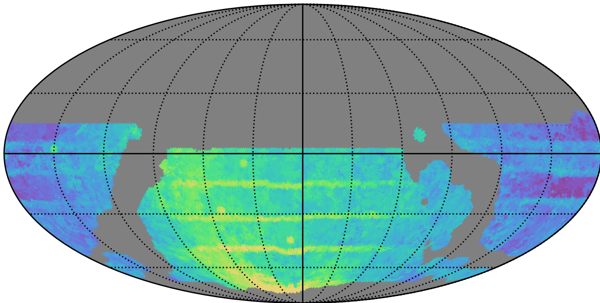
weather_cloudso20v3.4_10yrs WFD z band: Median Season Length
