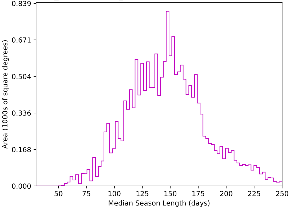
weather_cloudso20v3.4_10yrs WFD z band: Median Season Length
