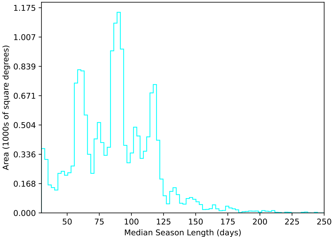
weather_cloudso20v3.4_10yrs WFD u band: Median Season Length
