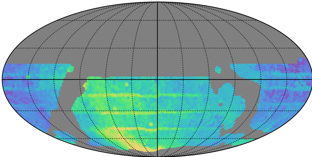
weather_cloudso20v3.4_10yrs WFD r band: Median Season Length
